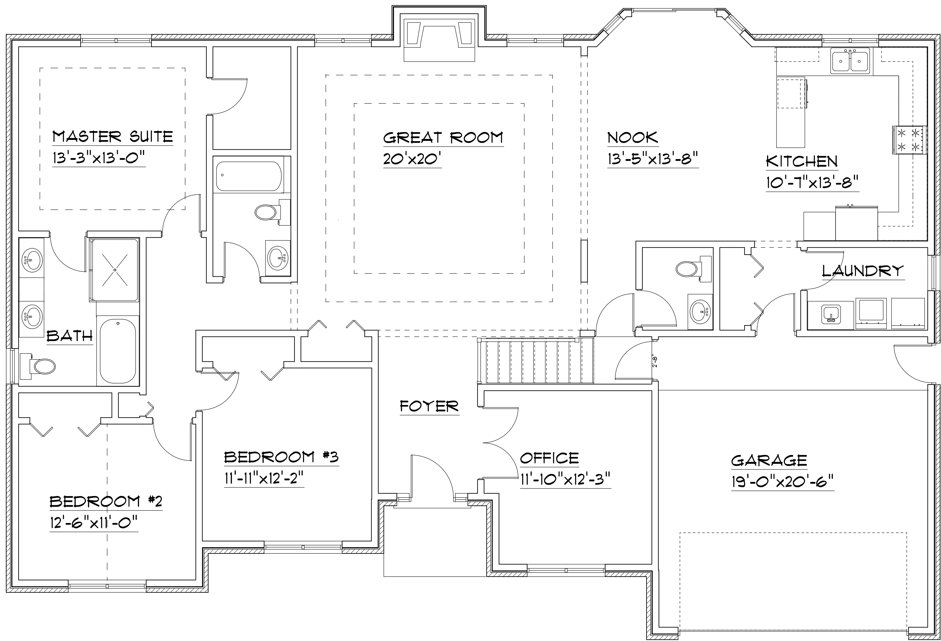
Main level Floor Plan 2094 Square Footage
