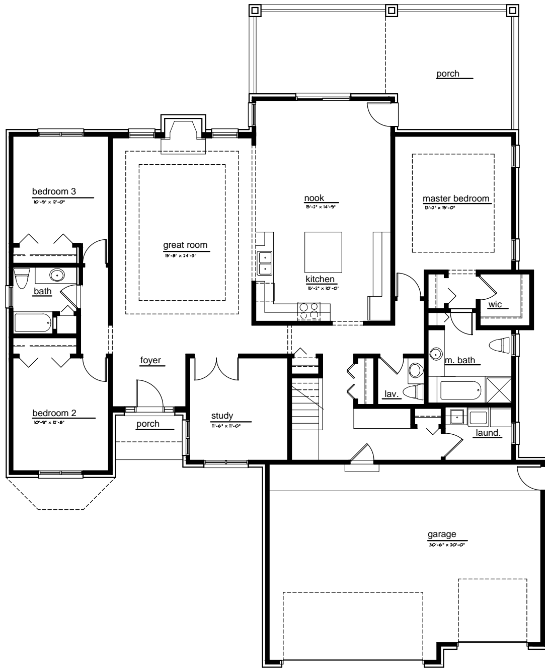
floor plan
